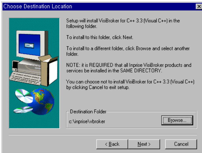
(visibrokerC++ 2.gif)
