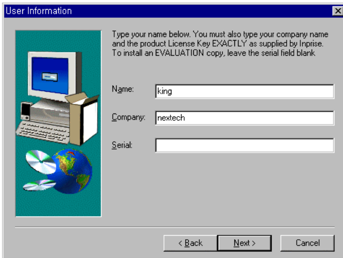
(visibrokerC++ 1.gif)
